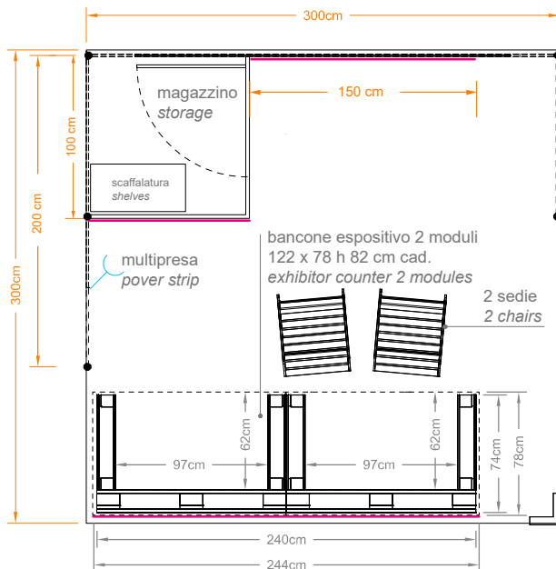
PIANTA / PLAN
